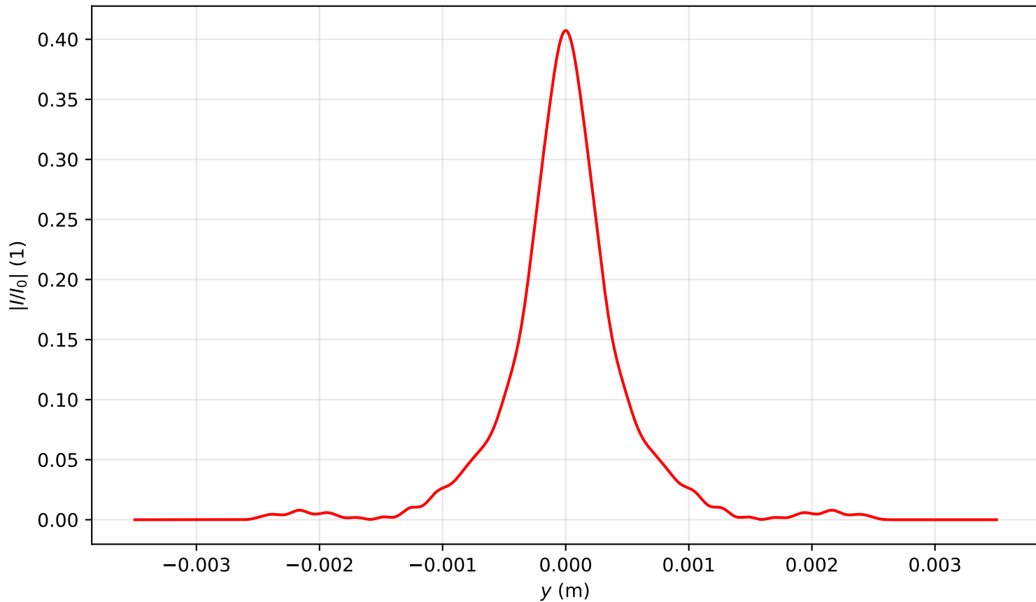
Intensity profile I(x=0, y, z=1.592)/I_0 , P_{in}=3.0P_{cr} , artificial time
